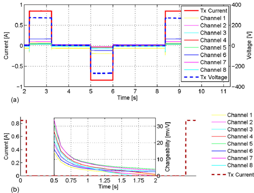
Fig. 3. (a) Terrameter LS transmitter current and voltage waveforms and input voltages from various input channels based on the 4 electrode configuration. (b) Induced polarisation decay curves from the various channels of the Terrameter LS measured during transmitter current off time.
