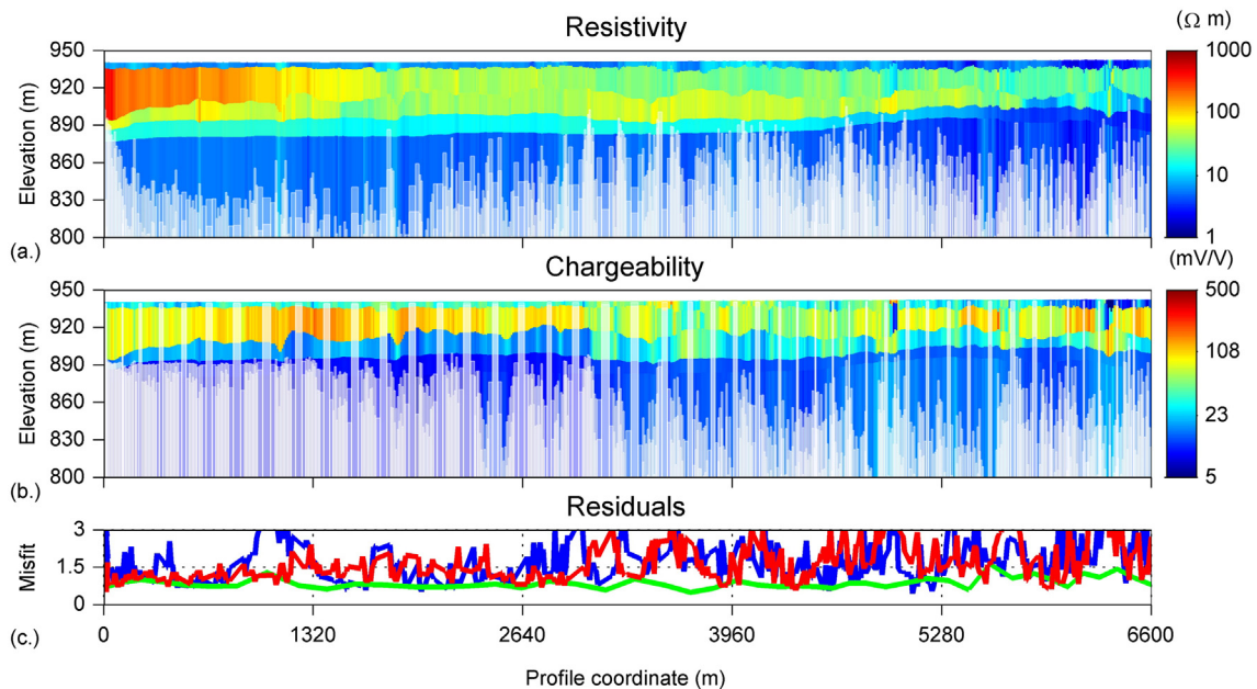
Fig. 7. (a) Inverse electrical resistivity cross section, (b) inverse chargeability cross section, and (c) data residual plot from joint inversion of DCIP and TEM data. The green line is for TEM residuals whereas the blue and red lines are for DC and IP residuals respectively.
