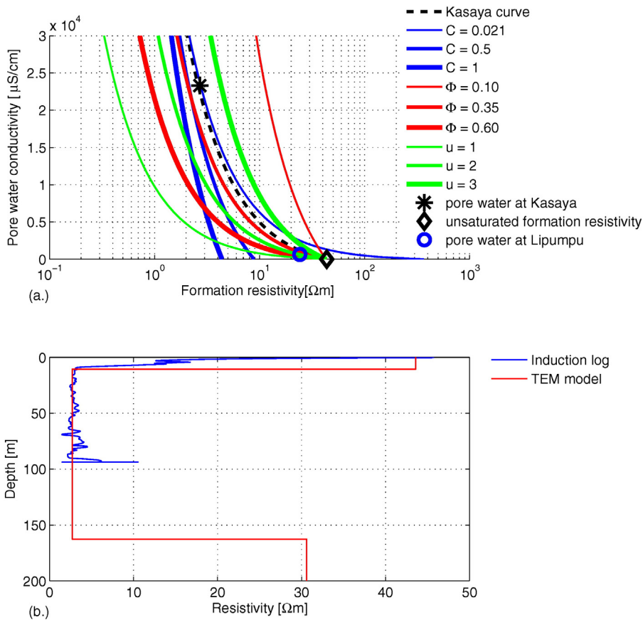
Fig. 5. (a) Illustration of the variation of the petro-physical relation (Eq. 1) for different parameters (porosity ( \phi ), volumetric water content exponent ( u ) and clay content ( C )). Kasaya curve is the curve fitting the measured borehole fluid conductivity at Kasaya and the unsaturated formation resistivity measured by TEM at the same location. (b) Variation of electrical resistivity with depth from an induction log and TEM sounding at Kasaya School in Machile–Zambezi Basin.
