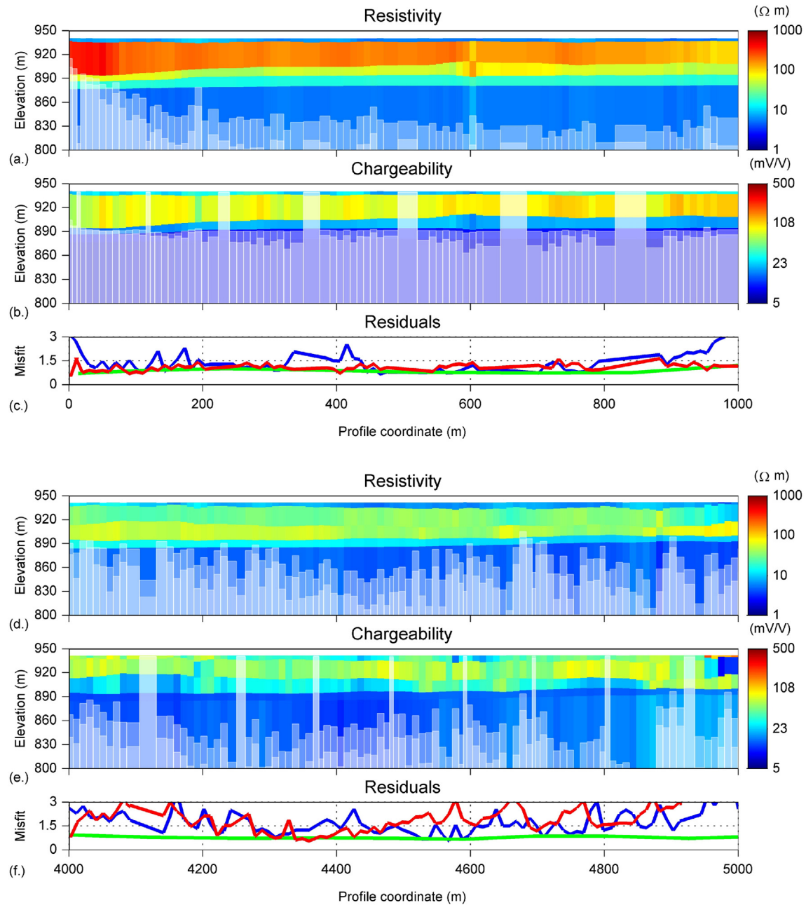
Fig. 8. (a)–(c) Zoom in inverse electrical resistivity cross section, inverse chargeability cross section, and data residual plot respectively from joint inversion of DCIP and TEM data for distance interval 0–1000 m. (e)–(f) Zoom in inverse electrical resistivity cross section, inverse chargeability cross section, and data residual plot respectively from joint inversion of DCIP and TEM data for distance interval 4000–5000 m.
