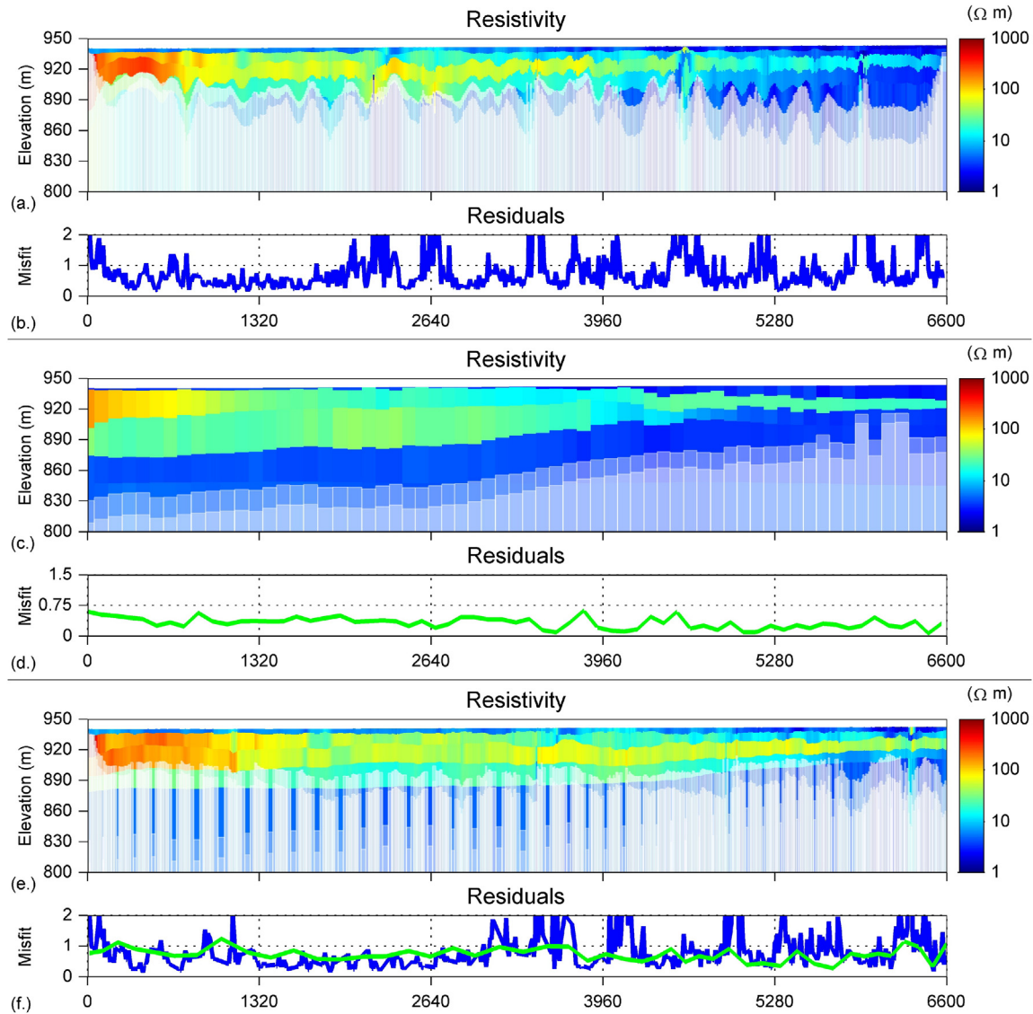
Fig. 6. Inverse electrical resistivity cross sections and residual plots. (a)–(b), Inverse electrical resistivity cross section and residual plot respectively for LCI of DC data; (c)–(d), inverse electrical resistivity cross section and residual plot respectively for LCI of TEM data; and (e)–(f), inverse electrical resistivity cross section and residual plot respectively for MCI-LCI (i.e. joint inversion) of DC and TEM data. On the residual plots, blue lines are for DC residuals whereas green lines are for TEM residuals.
