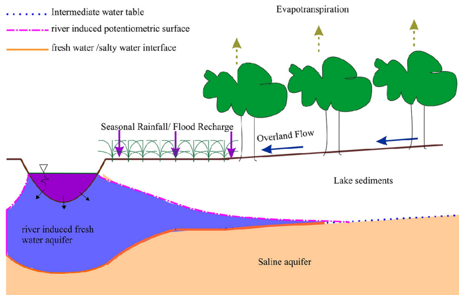
Fig. 9. Conceptual model of surface water/groundwater interaction in the Simalaha flood plain. The major drivers are conceptualised as seasonally varying water table in the Zambezi River, localised seasonal rainfall and flooding, overland flow and evapotranspiration.
