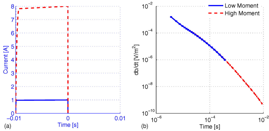
Fig. 4. (a) WalkTEM transmitter waveform and (b) typical earth response.
