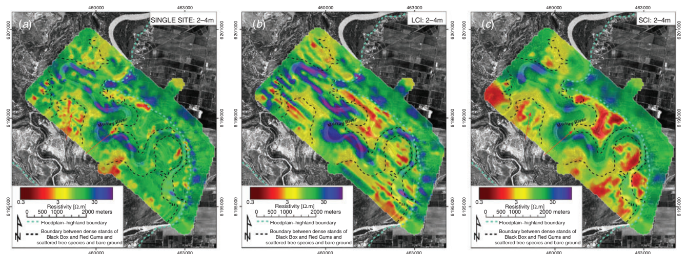
Fig. 10. Comparison between single site (a), laterally constrained inversion (LCI) (b) and spatially constrained inversion (SCI) (c) for resistivity depth interval 2–4 m below the ground surface. Red arrows indicate differences between single site and SCI results in resistive areas.
