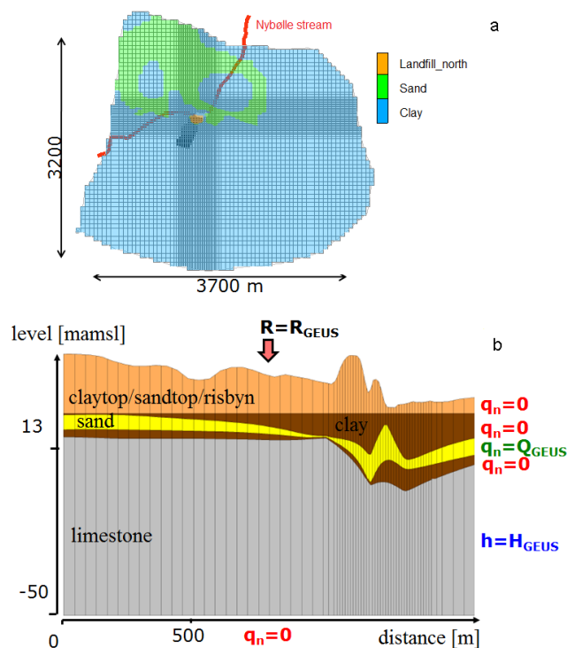
Fig. 7. Horizontal discretization of the Risby groundwater model and zonation of layer 1 (a) and the geological setup and boundary conditions used (b).
