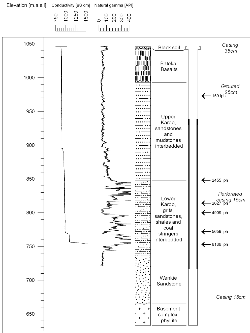
Fig. 4 Conductivity and natural gamma (Mangeya 2003) and summarized lithologic logs (MacDonald 1970) at borehole G3/463. The vertical scale is elevation in metres. To the right , the measured inflows from MacDonald (1970) are stated in litres per hour (lph). The location of the borehole is shown on Fig. 3
