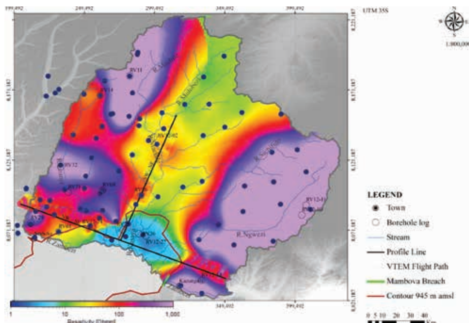
FIGURE 6 Mean horizontal electrical resistivity variations at depth interval 80 m–100 m.
