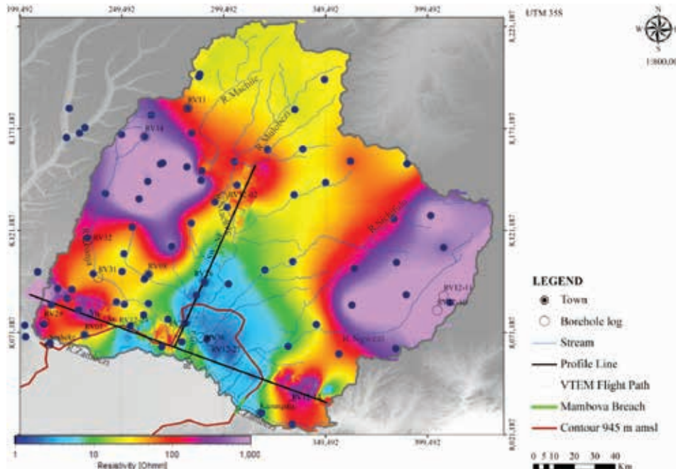
FIGURE 5 Mean horizontal electrical resistivity variations at depth interval of 0 m–20 m.
