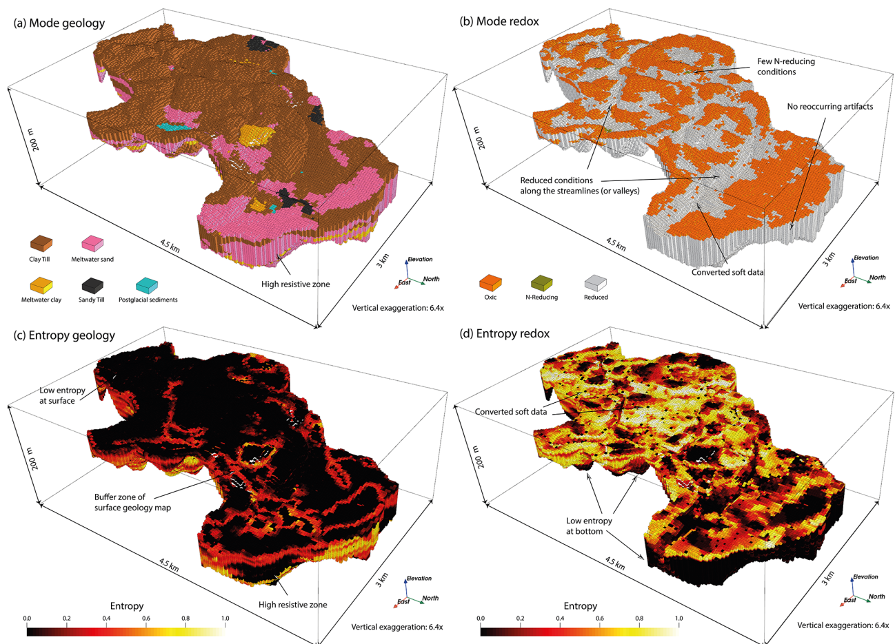
Figure 14. Mode and entropy of 100 geology and redox realizations. Low entropy (certainty) is marked with black color, while white colors represent high entropy (uncertainty).
